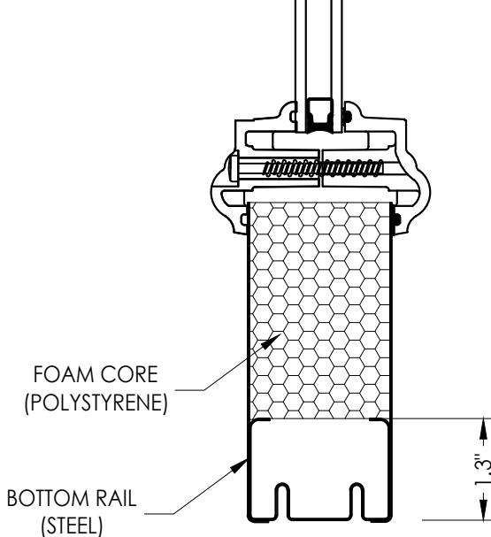
2 3 VERTICAL CROSS SECTION
